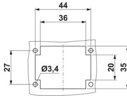
Mounting cut-out
