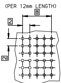
LAYOUT FOR P.C.B
